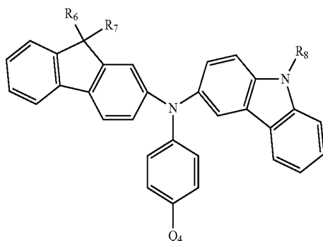
Formula 3a
