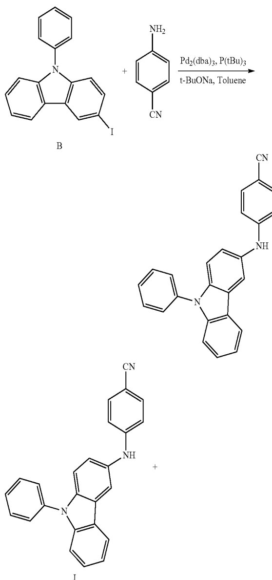
Reaction Scheme 8
