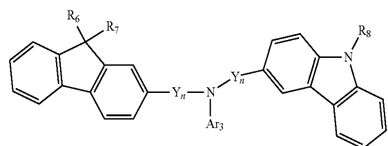
Formula 3
