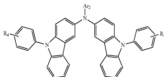
Formula 2
