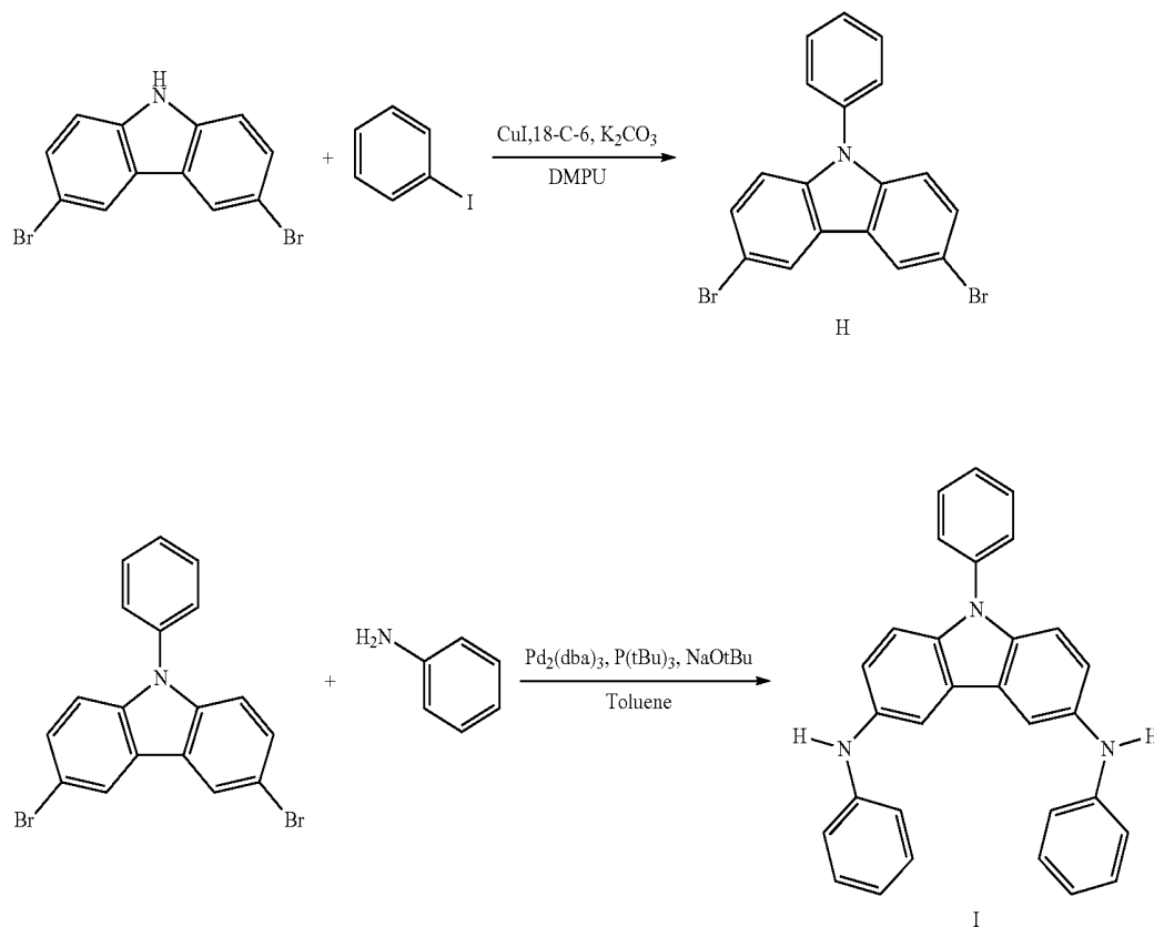
Reaction Scheme 7
